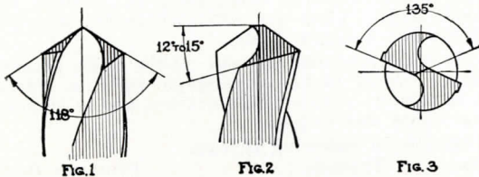
Cutting Edges Must Be of Equal Angle and of Equal Length Drills Grinding
